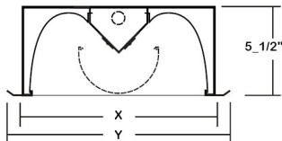
Ceiling Opening X - 12 1/2" x 48 1/2" Overall Width By Length Y - 14" x 50"
