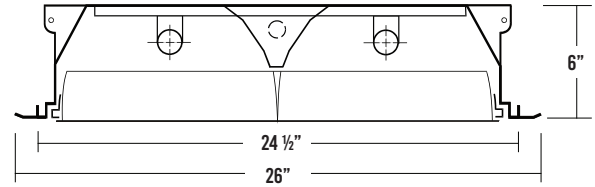
S12 CROSS SECTION
