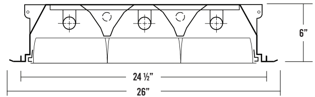
S18 CROSS SECTION
