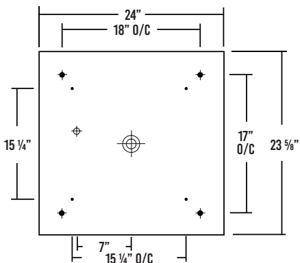
BACKPLATE
