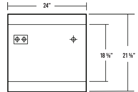
BACKPLATE
